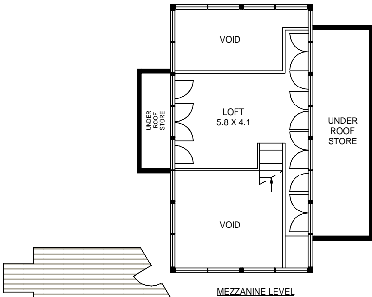
MEZZANINE LEVEL
